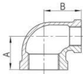
Reducing Elbow, 90°
