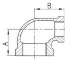
Reducing Elbow, 90°
